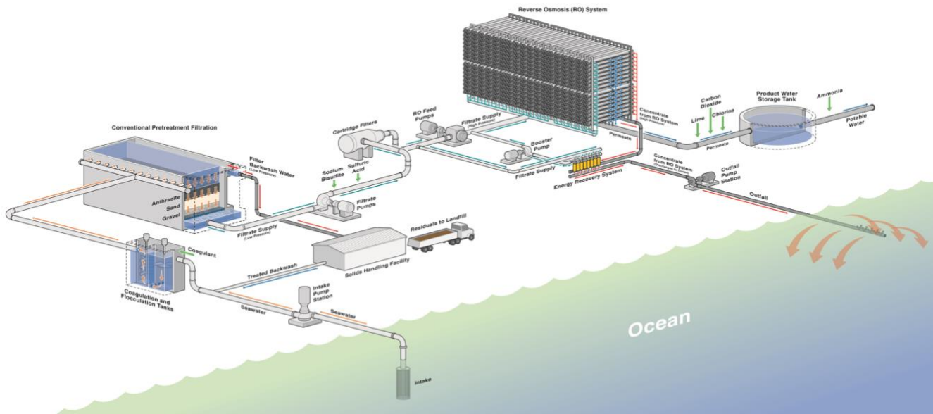
Figure 1 – Schematic of Typical Desalination Plant
