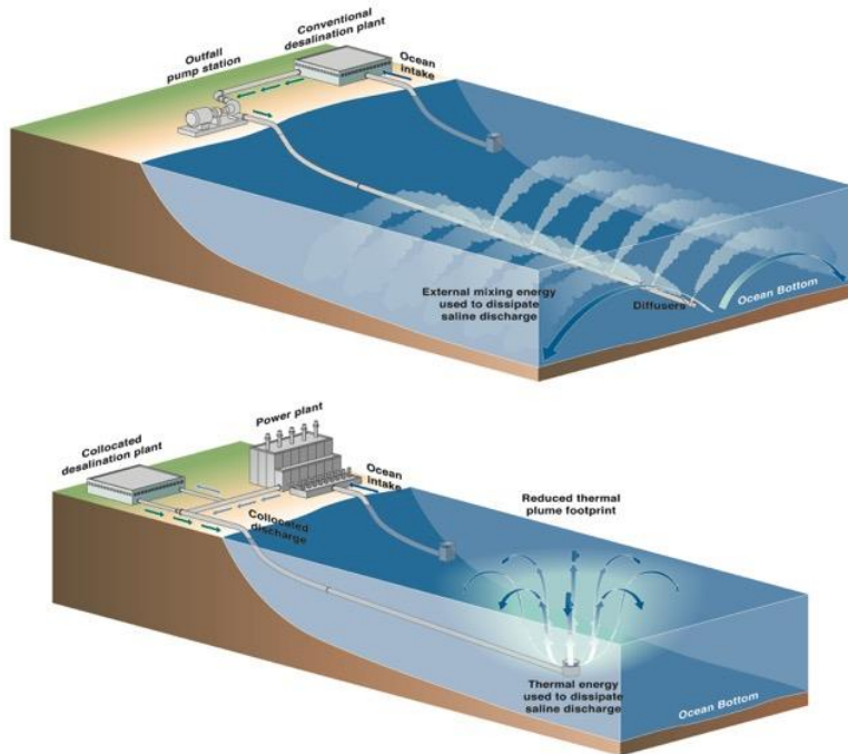
Figure 8 – Comparison of Concentrate Mixing Patterns of Collocated and New Outfalls
