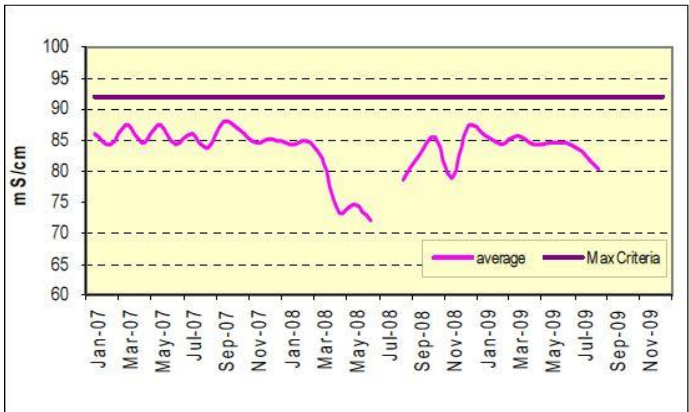
Figure 14 – Perth Desalination Plant – Discharge Conductivity
