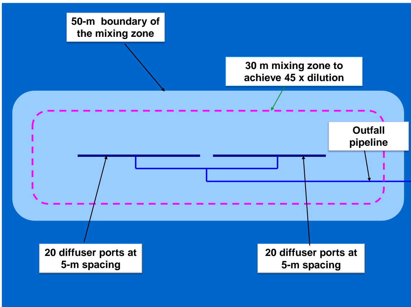
Figure 12 – Perth SWRO Plant Discharge Configuration
