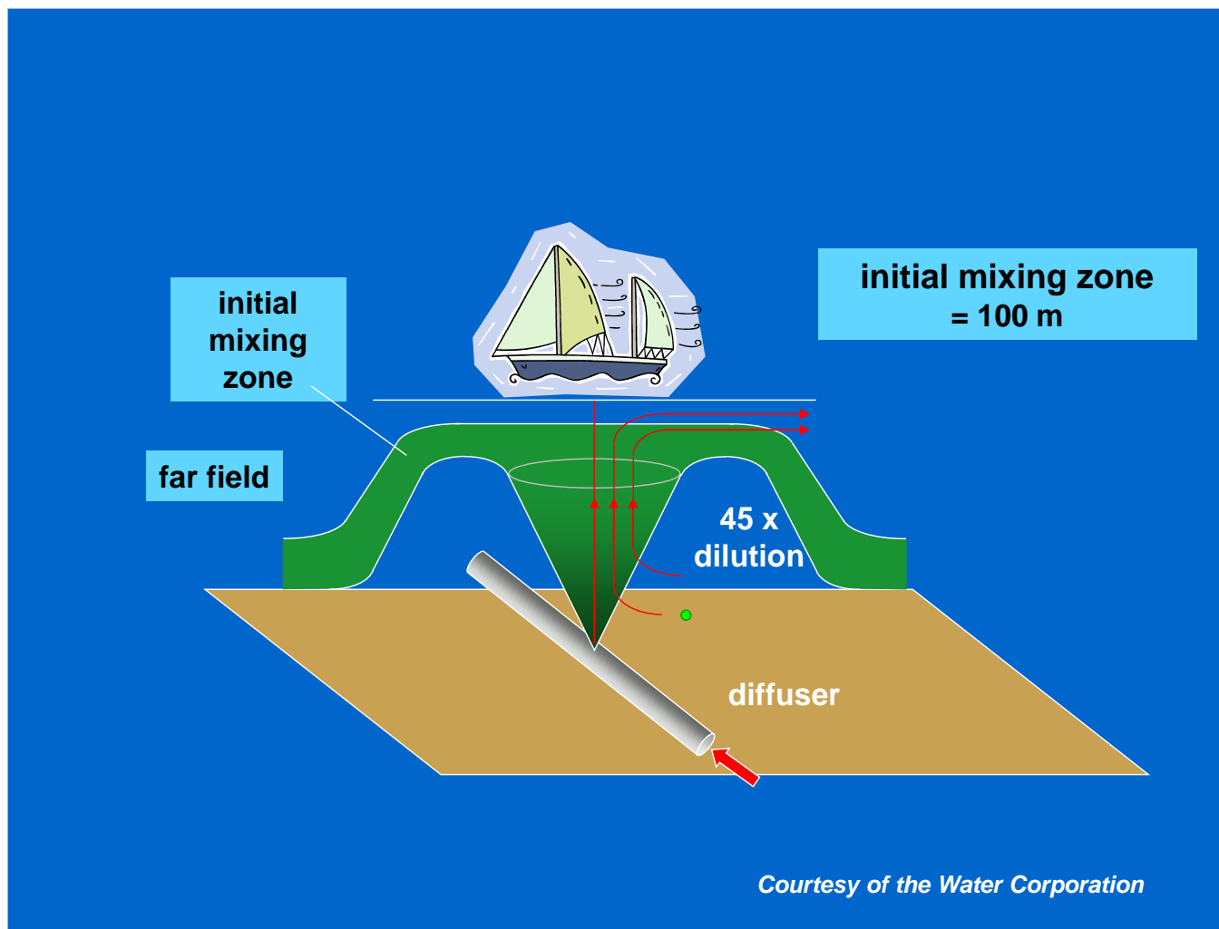
Figure 13 - Perth Desalination Plant Mixing Zone
