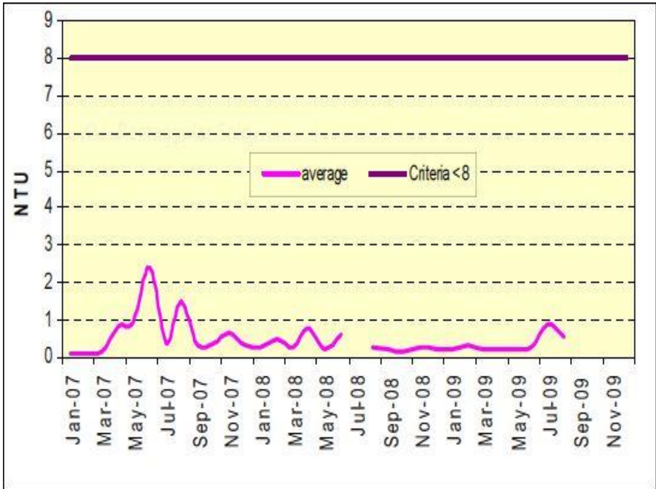
Figure 15 – Perth Desalination Plant – Discharge Turbidity
