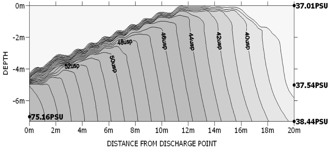
Figure 19 – Maspalomas SWRO Plant – Outfall Salinity Field
