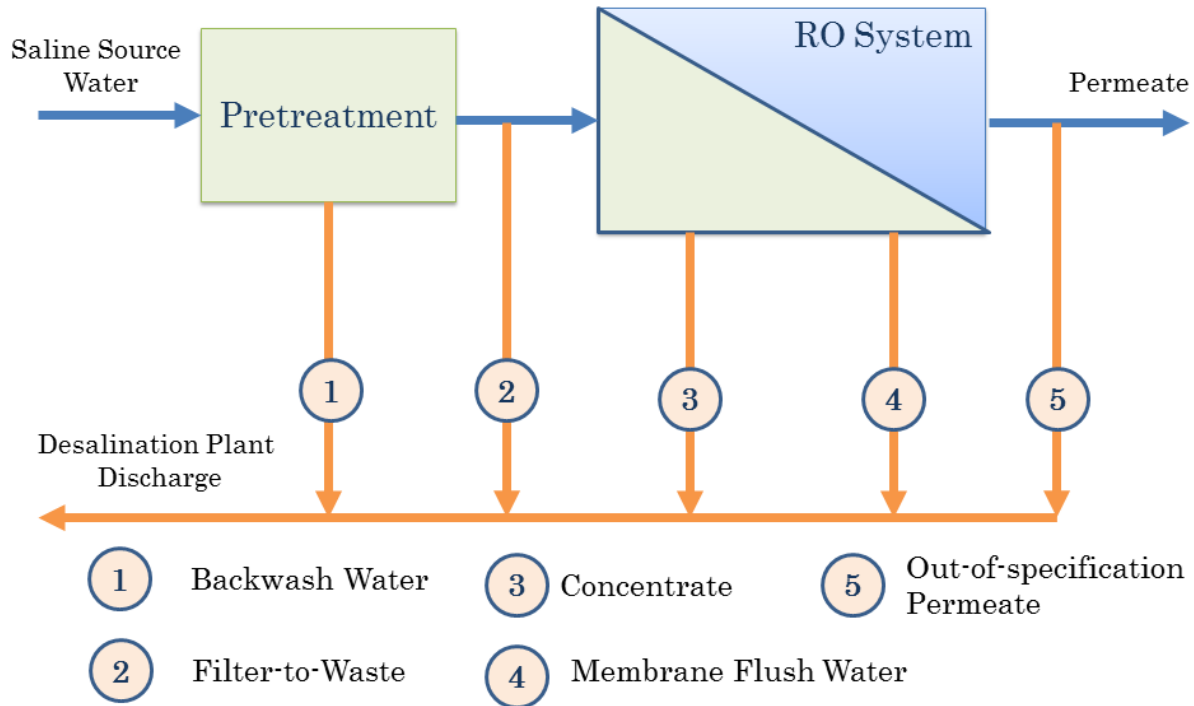
Figure 2 – Typical Discharge Components of Seawater Desalination Plant
