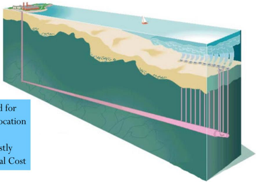
Figure 5 – New Ocean Outfall – Typical Configuration
